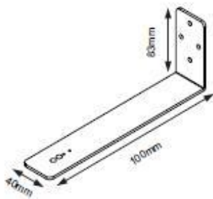
Wall Bracket
