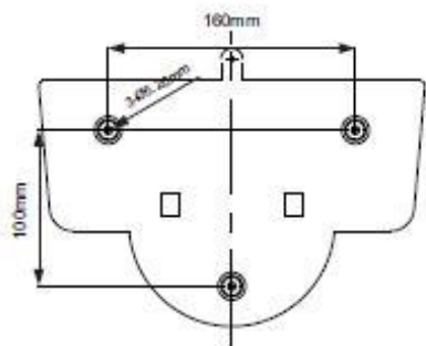
Ceiling Plate
